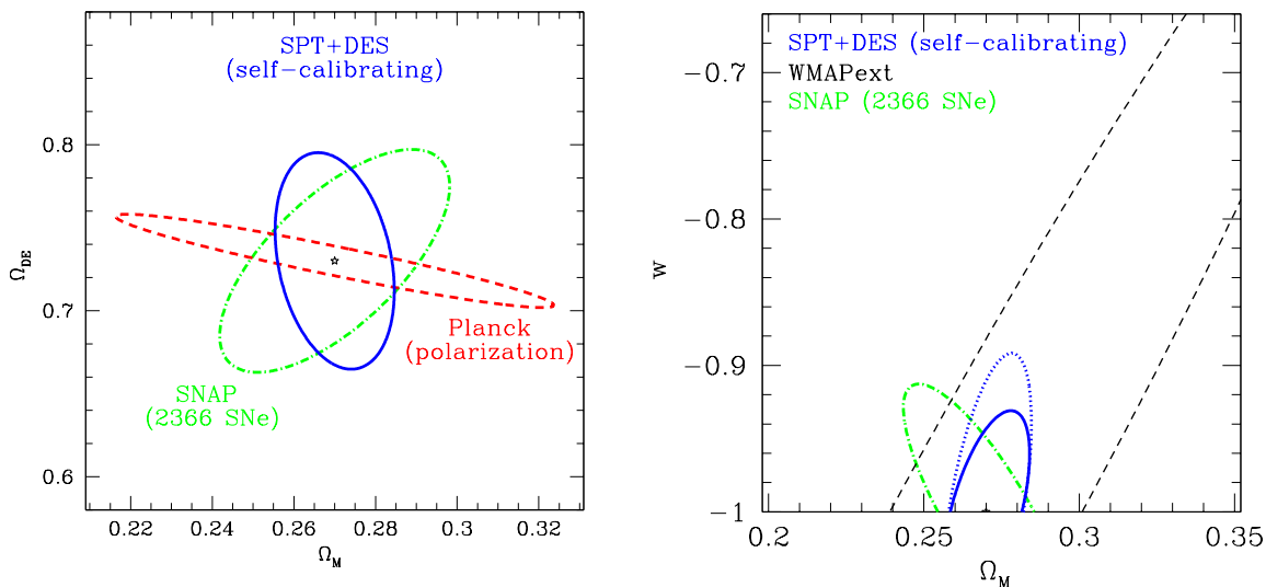
Figure 1: Forecasts for the geometry constraints (left) from the SPT+DES galaxy cluster survey, the SNAP SNe Ia mission, and the Planck CMB anisotropy mission together with forecasts for the joint \Omega_M - w constraints from the WMAP CMB anisotropy mission, SNAP and SPT+DES. These experiments are highly complementary because each experiment constrains a different combination of cosmological parameters and is subject to different systematics.
